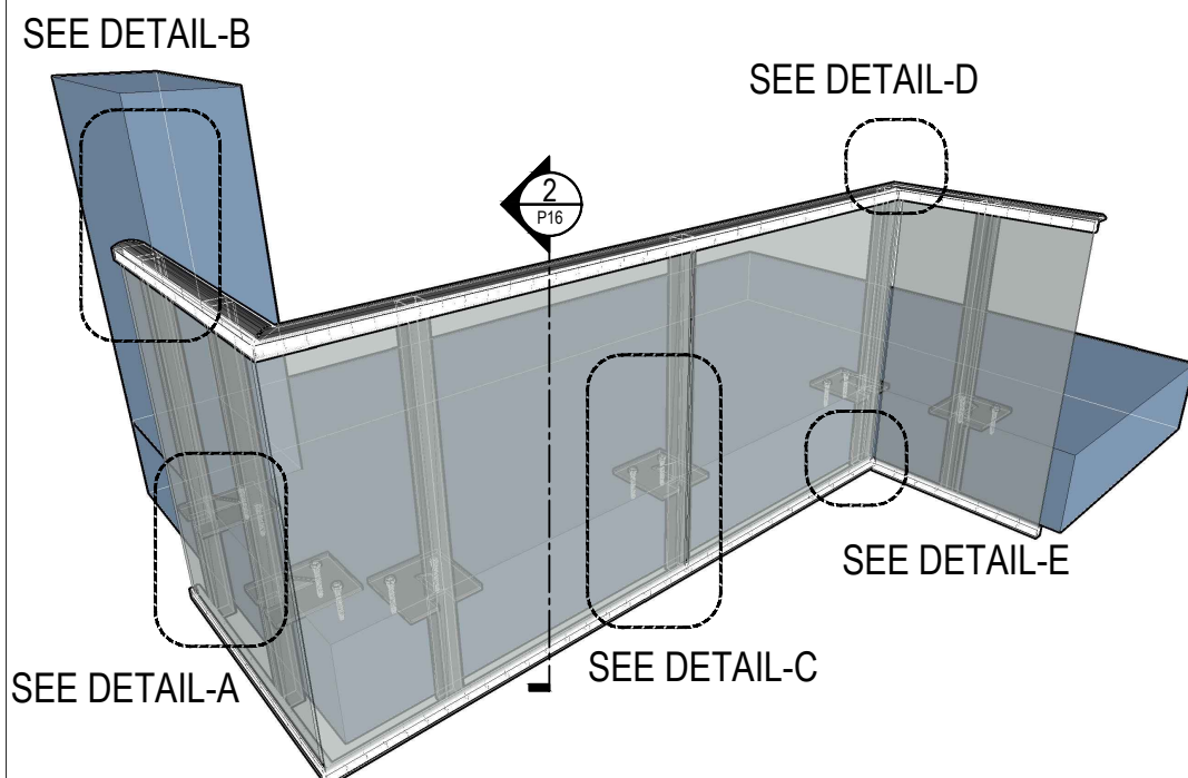
1 PERSPECTIVE P16 SCALE: NTS
